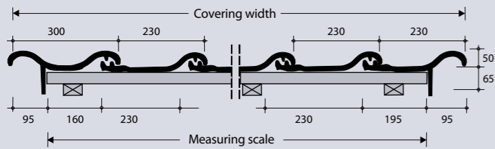
A: Verge tile with interior baulk
