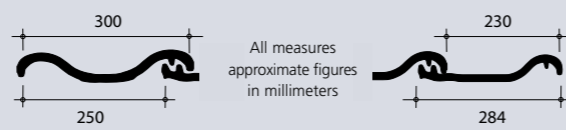
B: Double brim tile
